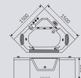
HX-0834 SIZE: 1500 X 1500 X 600 mm
