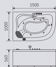
HX-0877R SIZE: 1500 X 1000 X 560 mm
