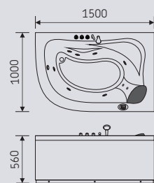
HX-0877L SIZE: 1500 X 1000 X 560 mm
