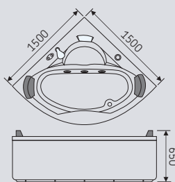
HX-0827 SIZE: 1500 X 1500 X 650 mm
