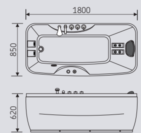
HX-0828 SIZE: 1800 X 850 X 620 mm
